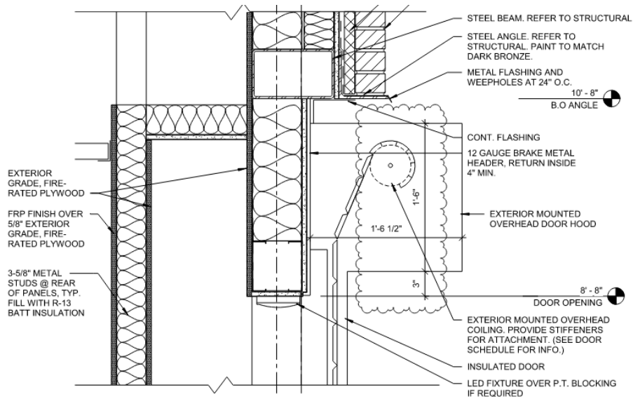
14 DETAIL - HEAD 04 1 1/2" = 1'-0"
